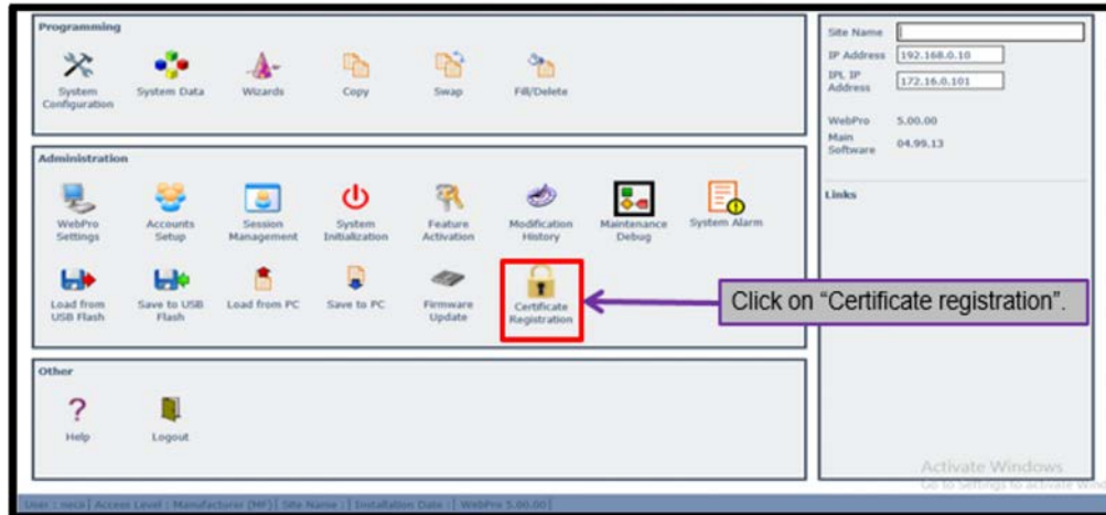
Figure 2-101 Certificate Registration
