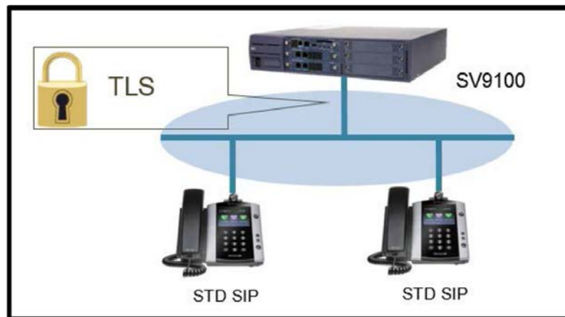
Figure 2-87 TLS Configuration
