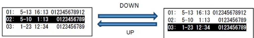
Figure 2-12 Scrolling – 3 Logs
