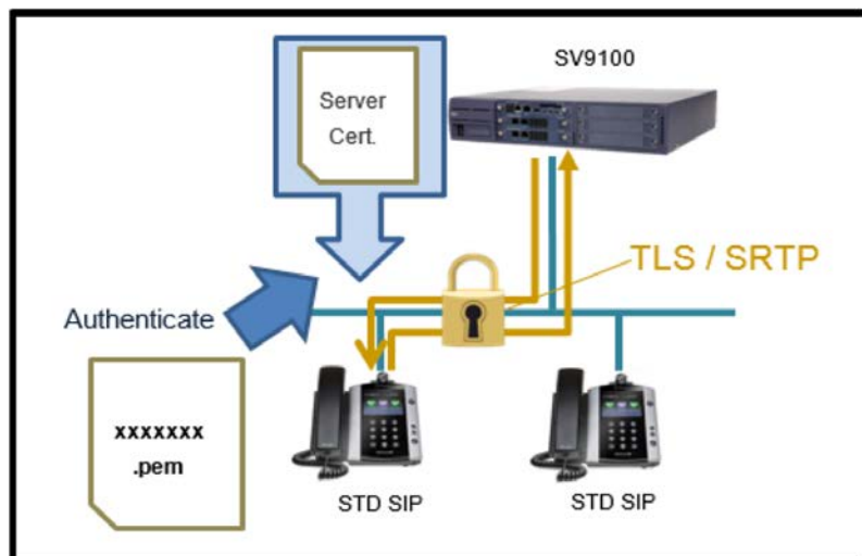
Figure 2-88 SV9100 Authentication
