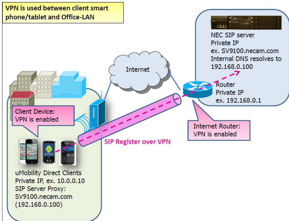
Figure 2-155 VPN Between Smart Device and Office LAN
