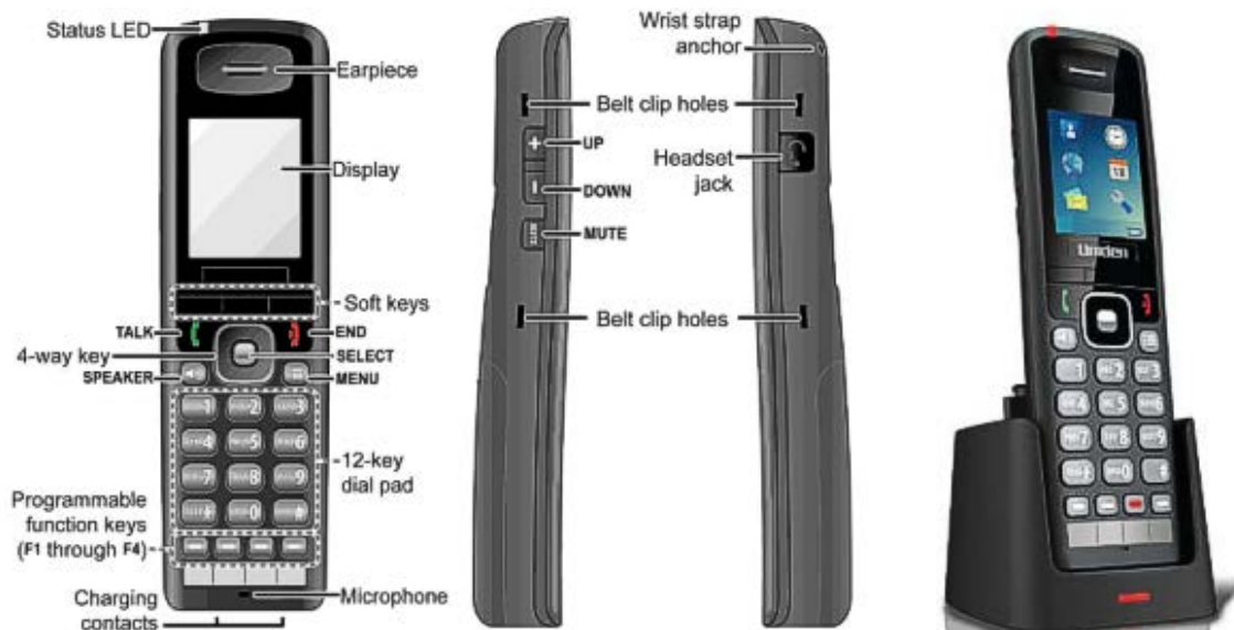
Figure 2-79 ML440 Cordless Handset
