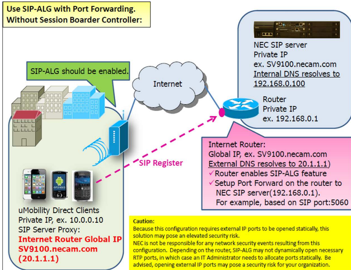
Figure 2-156 Port Forwarding without Session Border Controller
