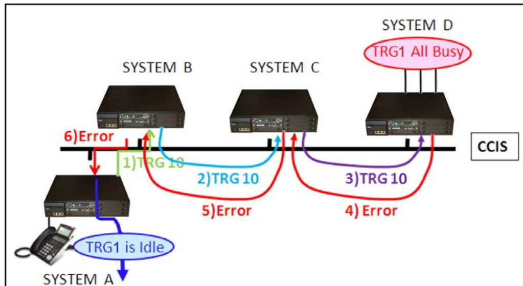
Figure 2-111 K-CCIS Call Rerouting Network
