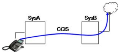
Figure 2-51 CCIS 911 Calls
