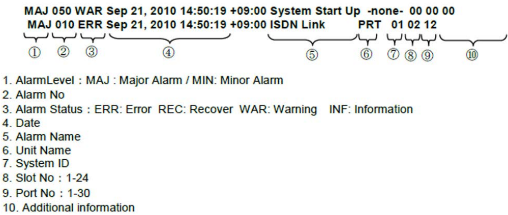
Figure 2-140 SNMP – Trap Alarm Details
