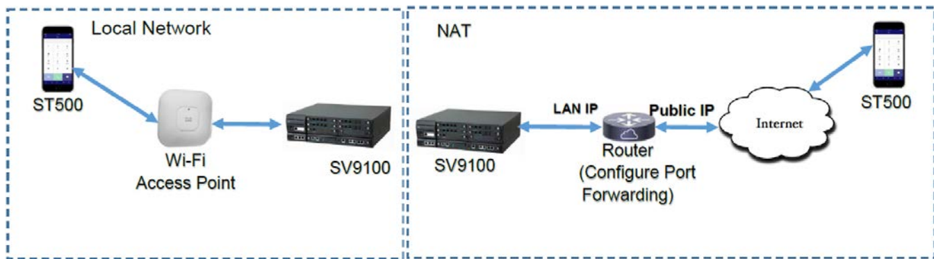
Figure 2-93 Example of ST500 on Local Network/NAT
