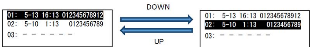
Figure 2-13 Scrolling – 2 Logs
